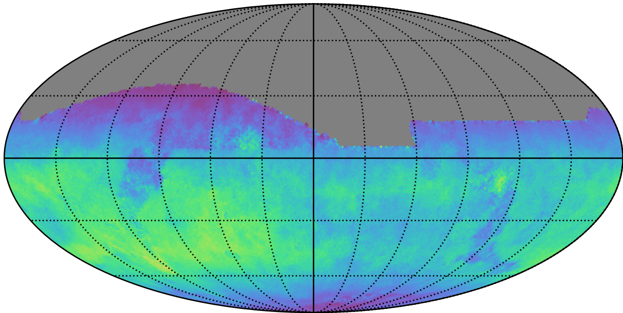
too_elab_r256_d2_griz_v3.4_10yrs All sky z band: Normalized Teff
