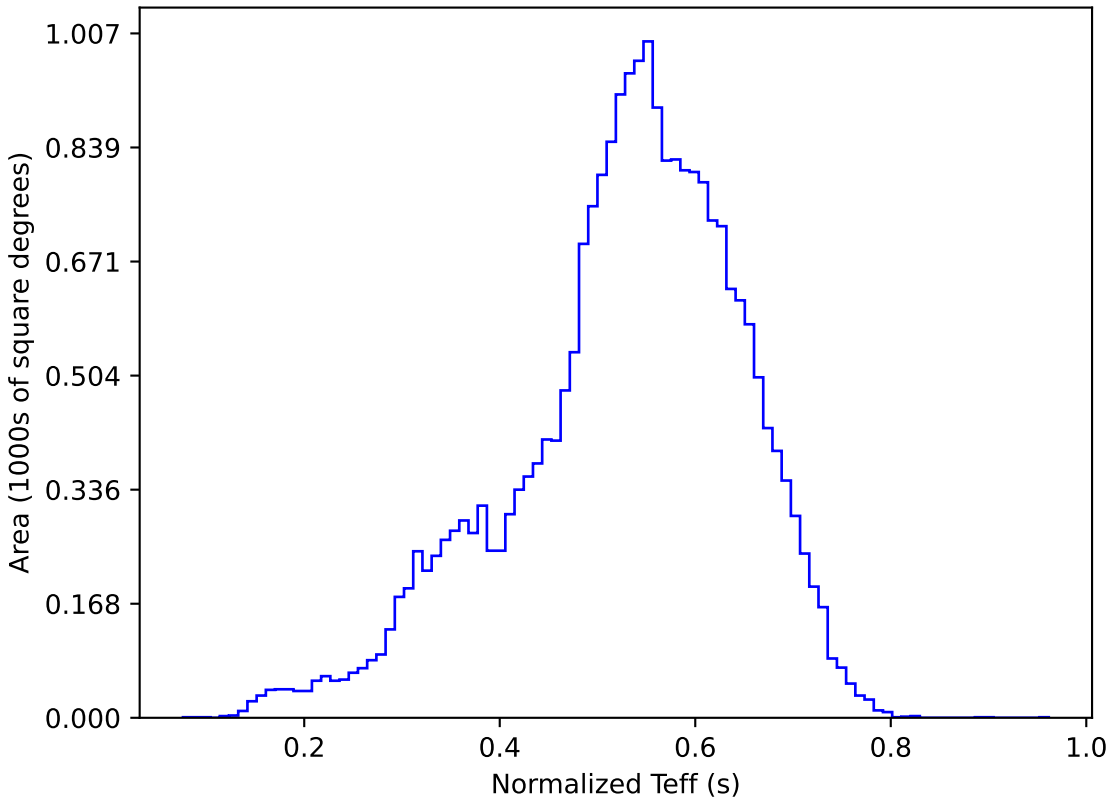
too_elab_r256_d2_griz_v3.4_10yrs All sky y band: Normalized Teff
