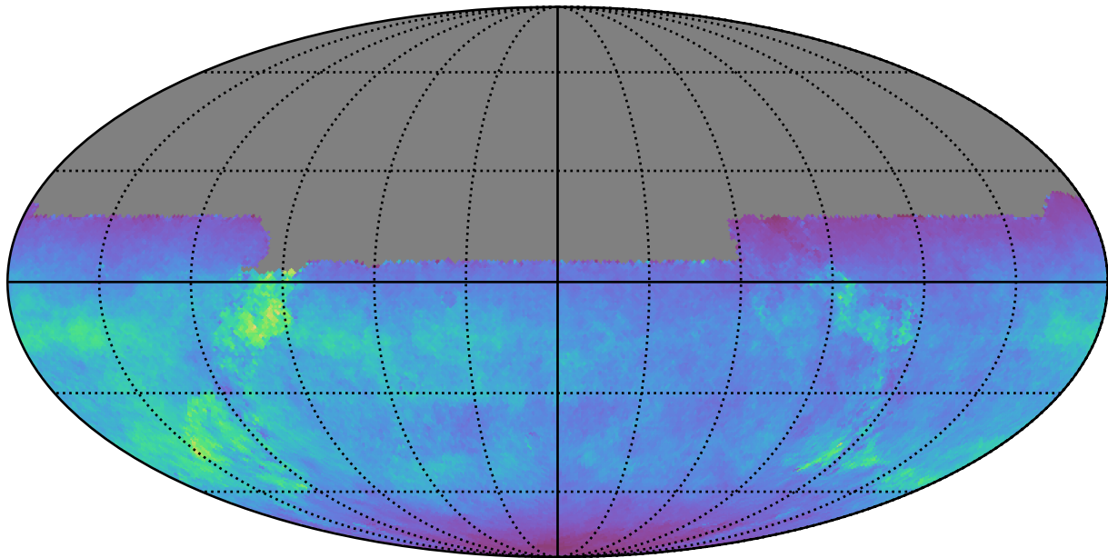
too_elab_r256_d2_griz_v3.4_10yrs All sky u band: Normalized Teff
