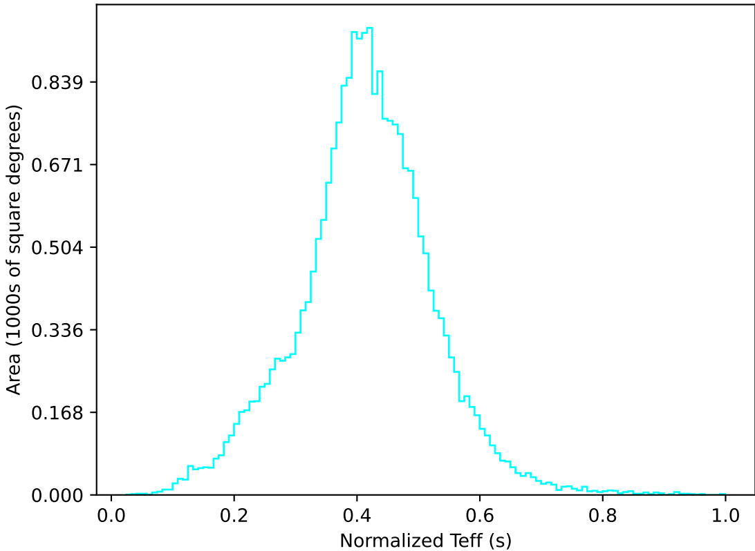
too_elab_r256_d2_griz_v3.4_10yrs All sky u band: Normalized Teff
