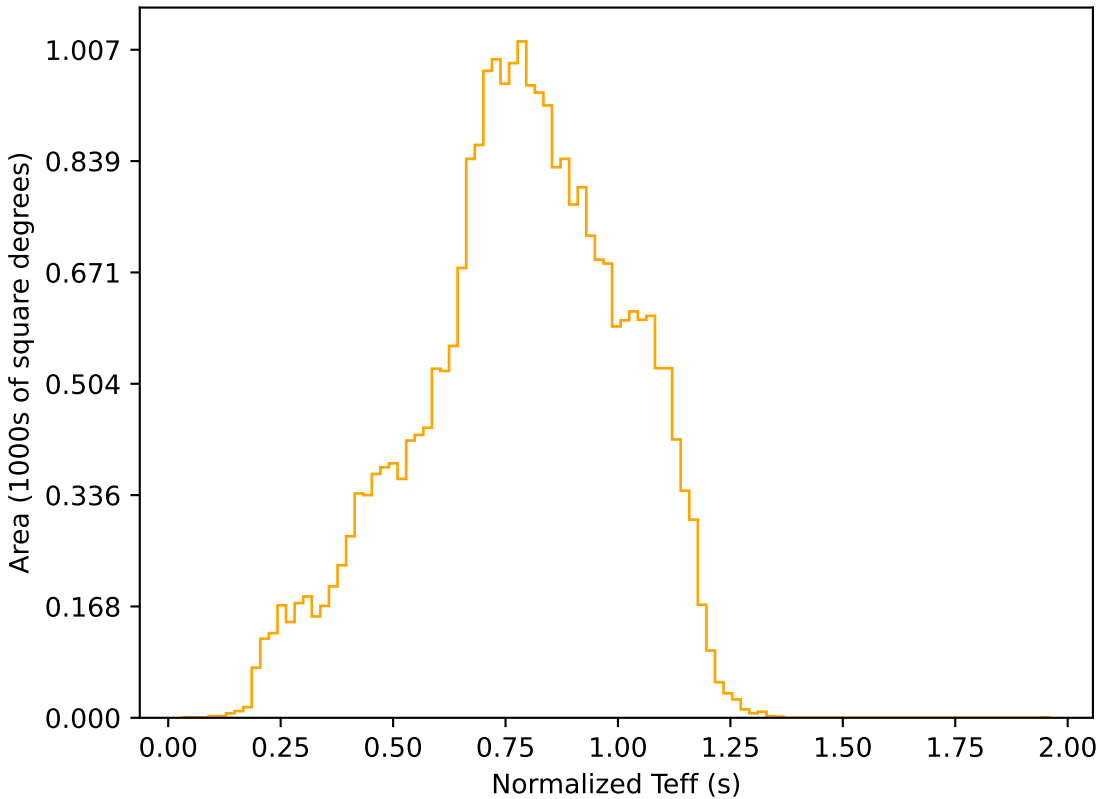
too_elab_r256_d2_griz_v3.4_10yrs All sky r band: Normalized Teff
