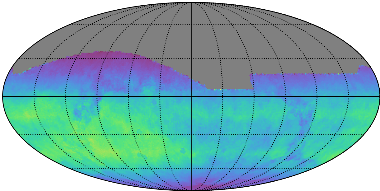
too_elab_r256_d2_griz_v3.4_10yrs All sky i band: Normalized Teff
