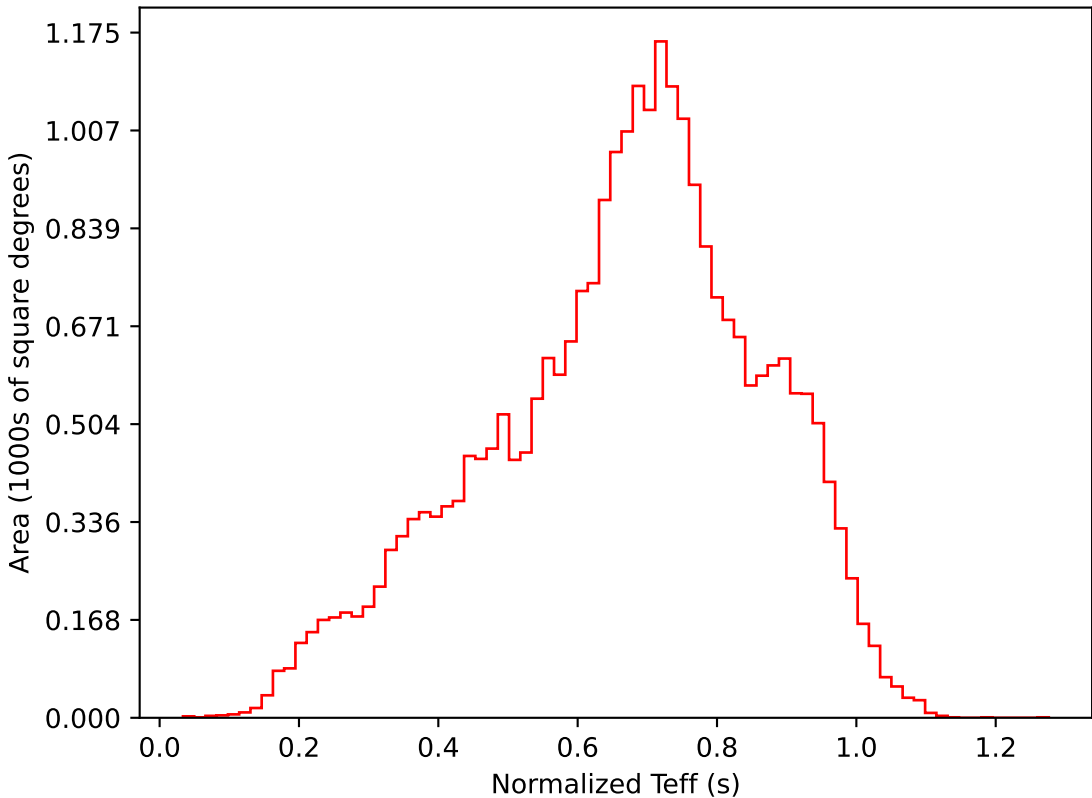
too_elab_r256_d2_griz_v3.4_10yrs All sky i band: Normalized Teff
