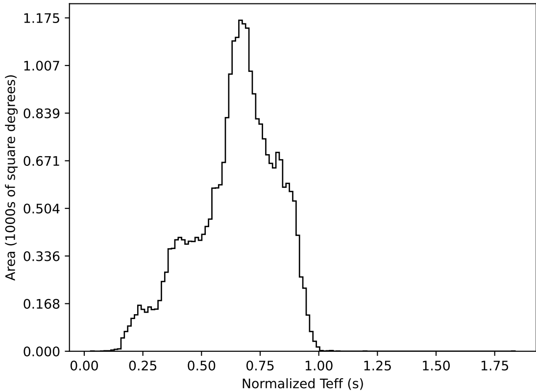
too_elab_r256_d2_griz_v3.4_10yrs All sky all bands: Normalized Teff
