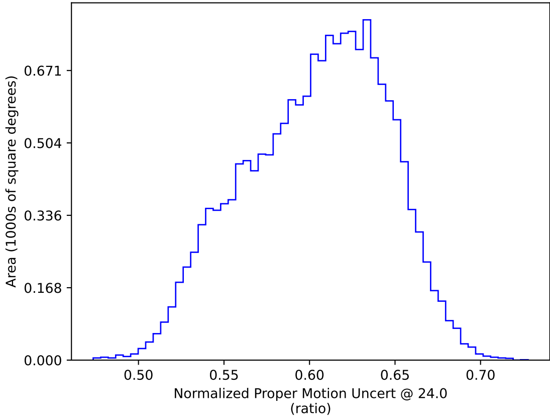
too_elab_r256_d2_griz_v3.4_10yrs WFD: Normalized Proper Motion Uncert @ 24.0
