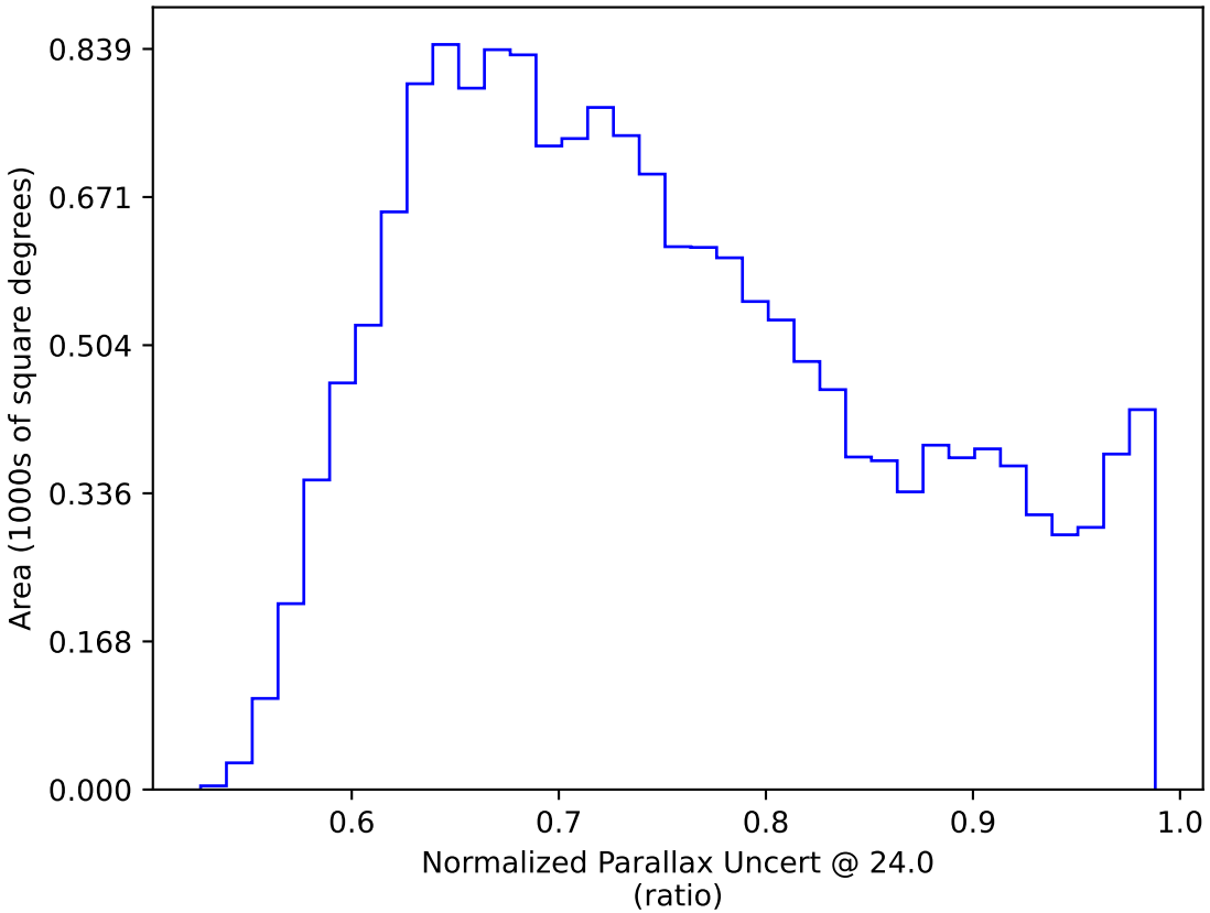
too_elab_r256_d2_griz_v3.4_10yrs WFD: Normalized Parallax Uncert @ 24.0
