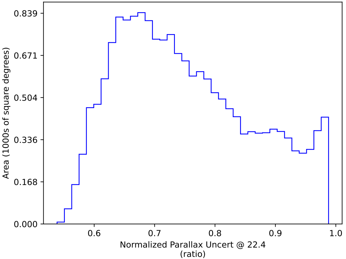
too_elab_r256_d2_griz_v3.4_10yrs WFD: Normalized Parallax Uncert @ 22.4
