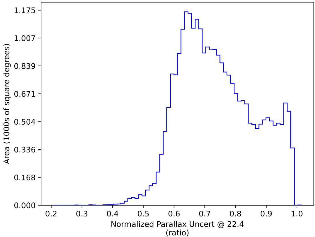
too_elab_r256_d2_griz_v3.4_10yrs All sky: Normalized Parallax Uncert @ 22.4
