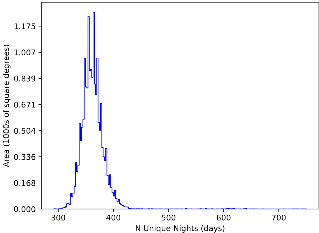
too_elab_r256_d2_griz_v3.4_10yrs WFD all bands: N Unique Nights
