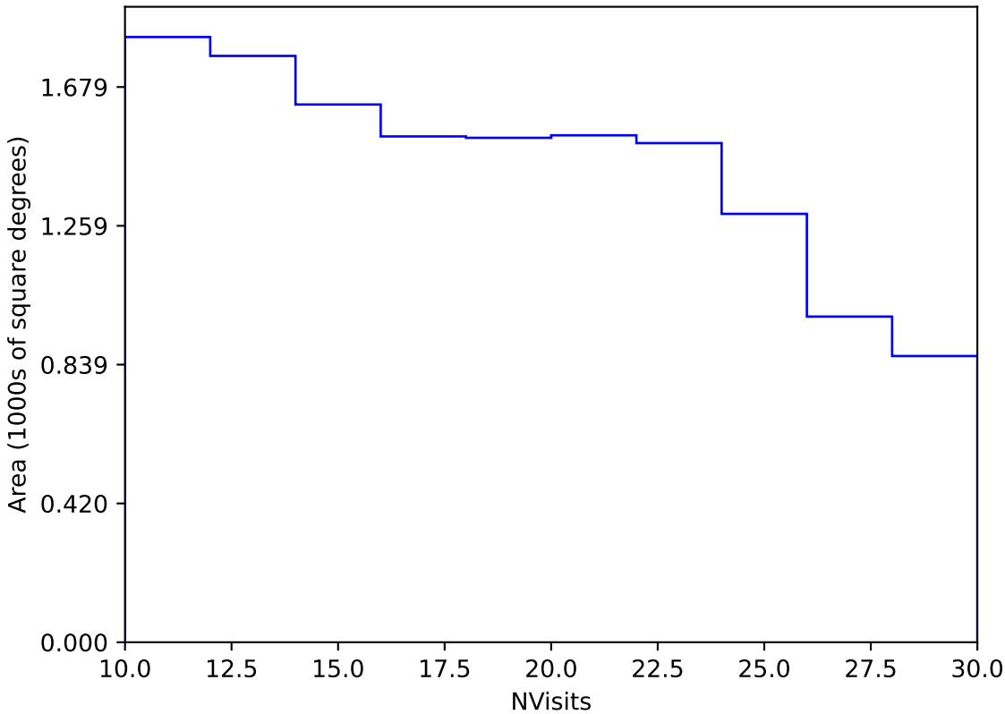
too_elab_r256_d2_griz_v3.4_10yrs Yr 3-4 y band: NVisits
