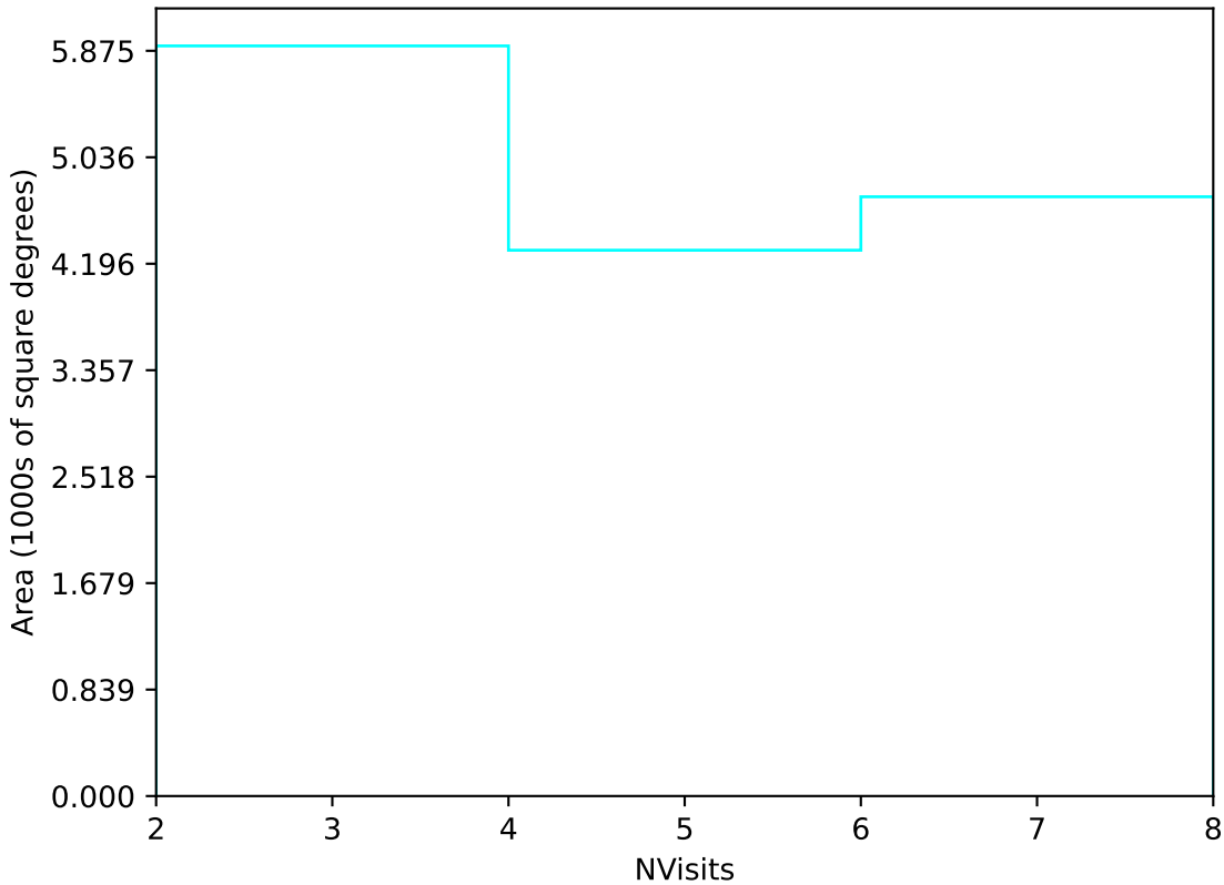
too_elab_r256_d2_griz_v3.4_10yrs Yr 3-4 u band: NVisits
