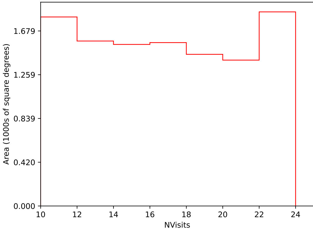
too_elab_r256_d2_griz_v3.4_10yrs Yr 3-4 i band: NVisits
