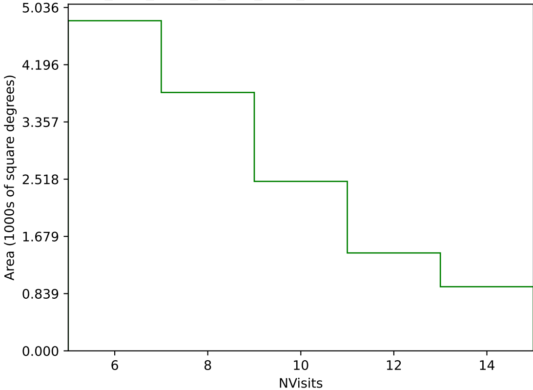
too_elab_r256_d2_griz_v3.4_10yrs Yr 3-4 g band: NVisits
