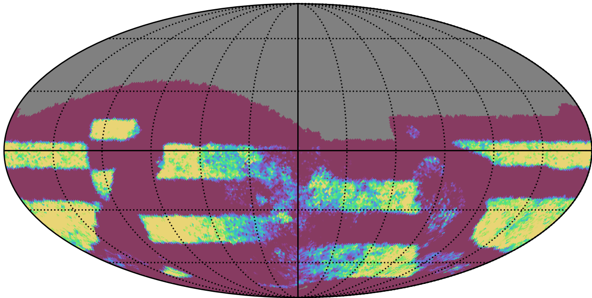
too_elab_r256_d2_griz_v3.4_10yrs Yr 3-4 all bands: NVisits
