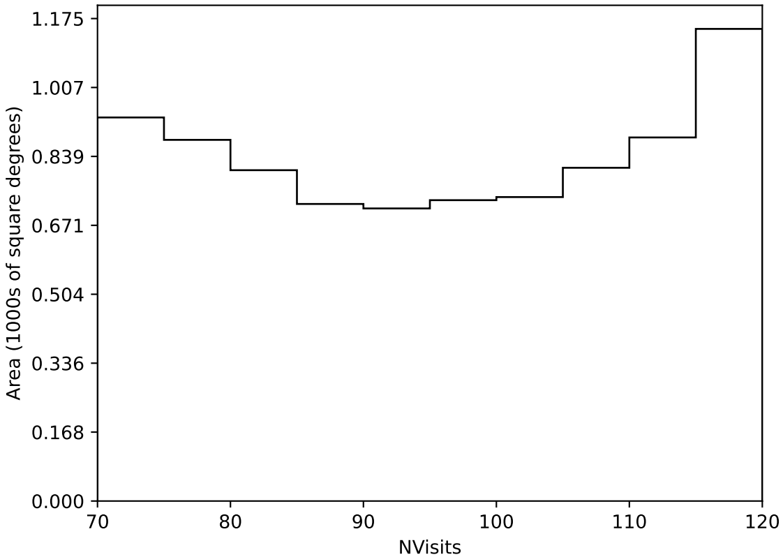
too_elab_r256_d2_griz_v3.4_10yrs Yr 3-4 all bands: NVisits
