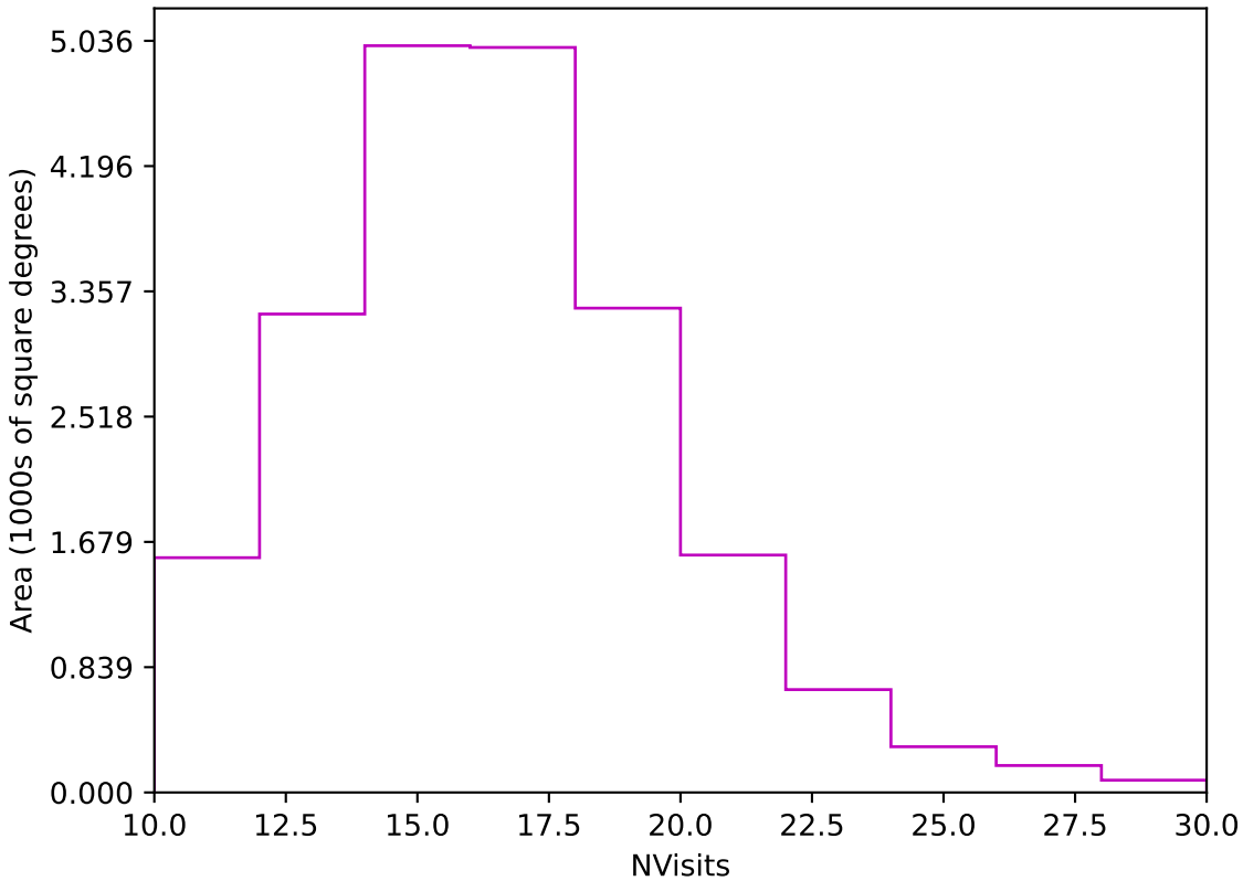
too_elab_r256_d2_griz_v3.4_10yrs Yr 1 z band: NVisits
