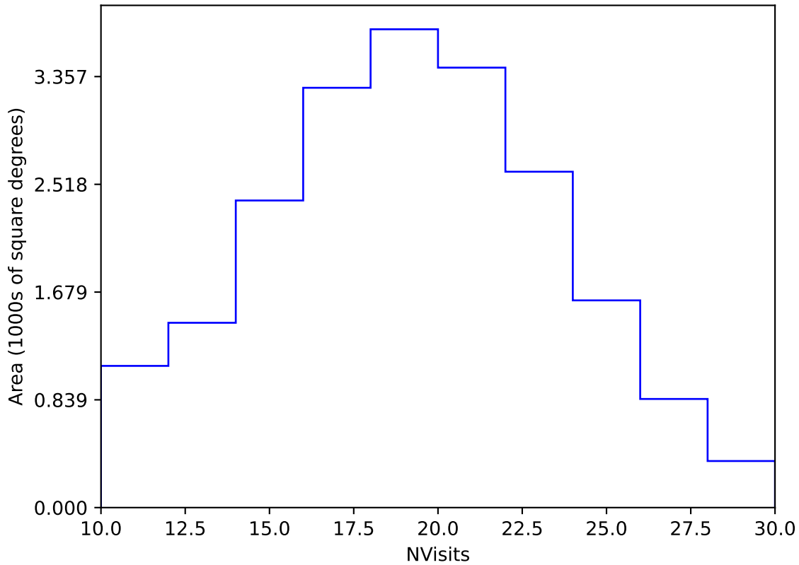
too_elab_r256_d2_griz_v3.4_10yrs Yr 1 y band: NVisits
