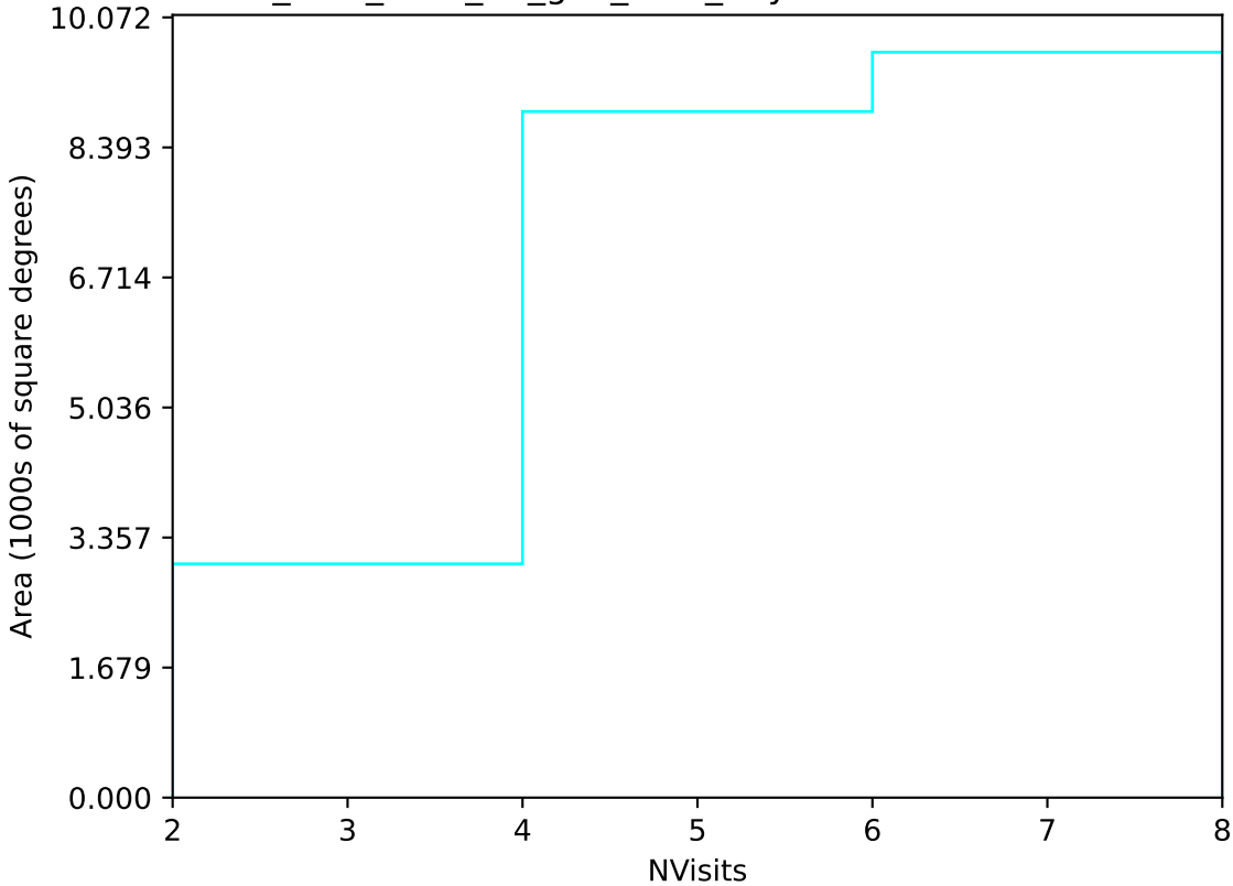
too_elab_r256_d2_griz_v3.4_10yrs Yr 1 u band: NVisits
