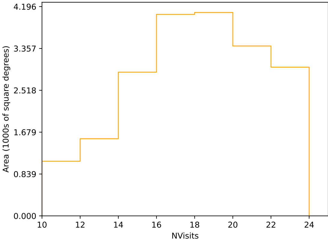
too_elab_r256_d2_griz_v3.4_10yrs Yr 1 r band: NVisits
