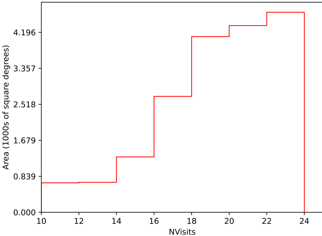
too_elab_r256_d2_griz_v3.4_10yrs Yr 1 i band: NVisits
