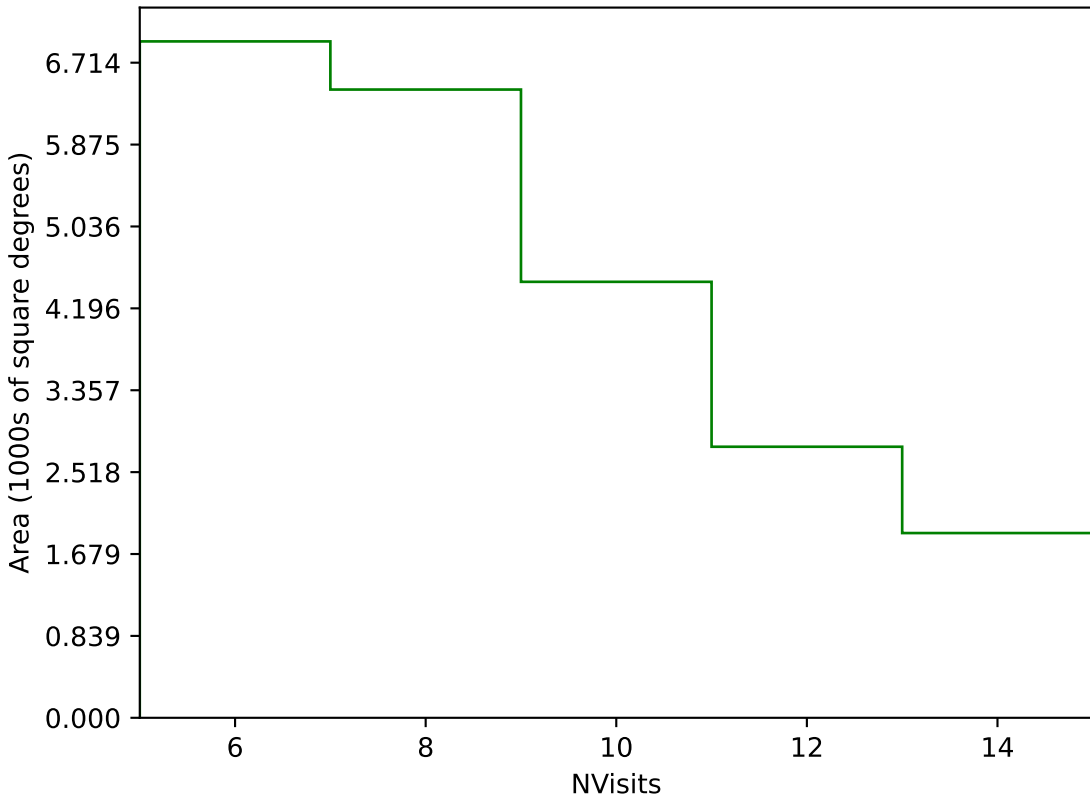
too_elab_r256_d2_griz_v3.4_10yrs Yr 1 g band: NVisits
