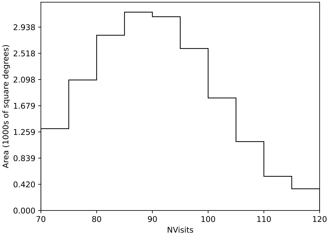
too_elab_r256_d2_griz_v3.4_10yrs Yr 1 all bands: NVisits
