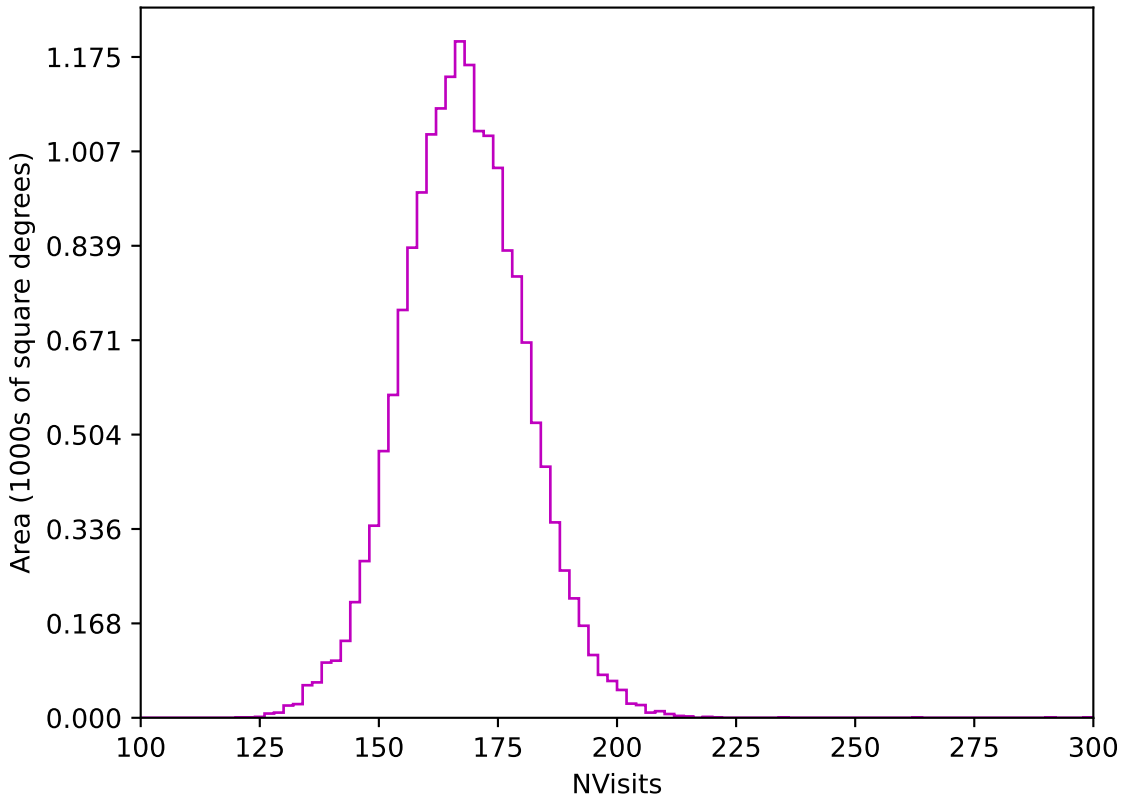
too_elab_r256_d2_griz_v3.4_10yrs WFD z band: NVisits
