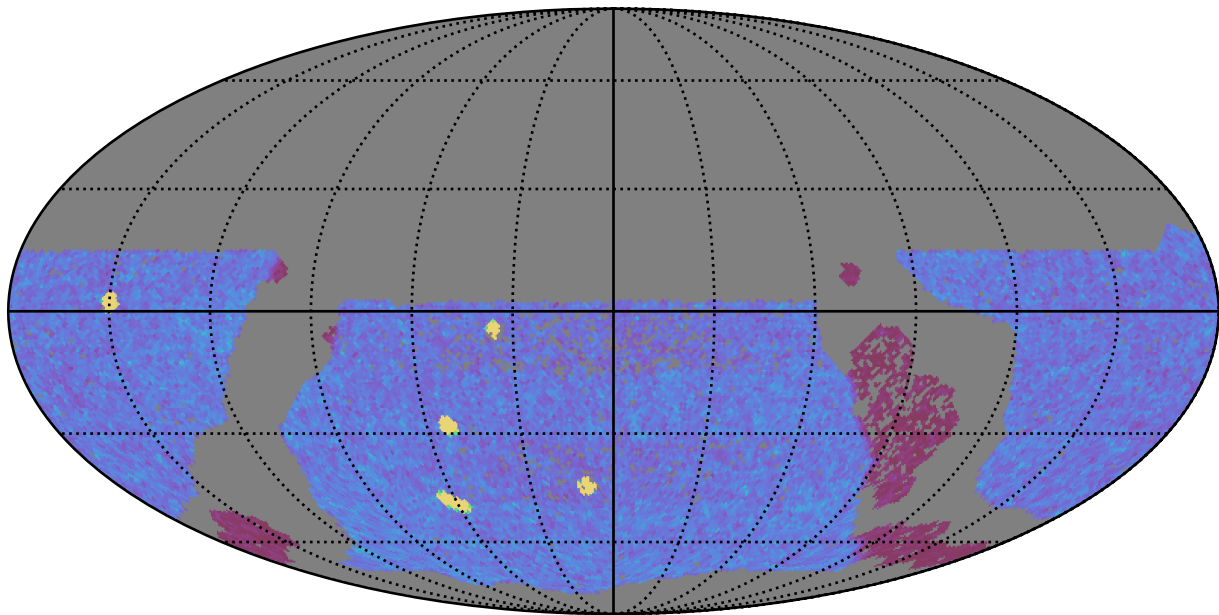
too_elab_r256_d2_griz_v3.4_10yrs WFD y band: NVisits
