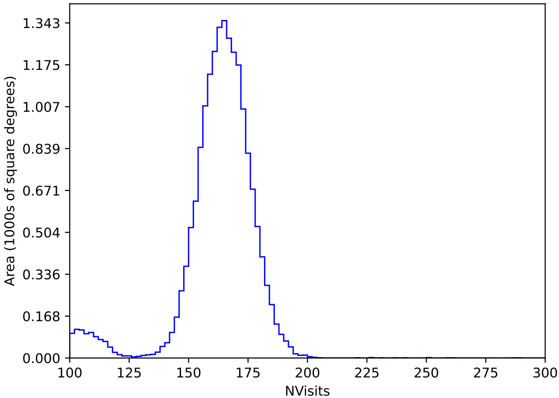
too_elab_r256_d2_griz_v3.4_10yrs WFD y band: NVisits
