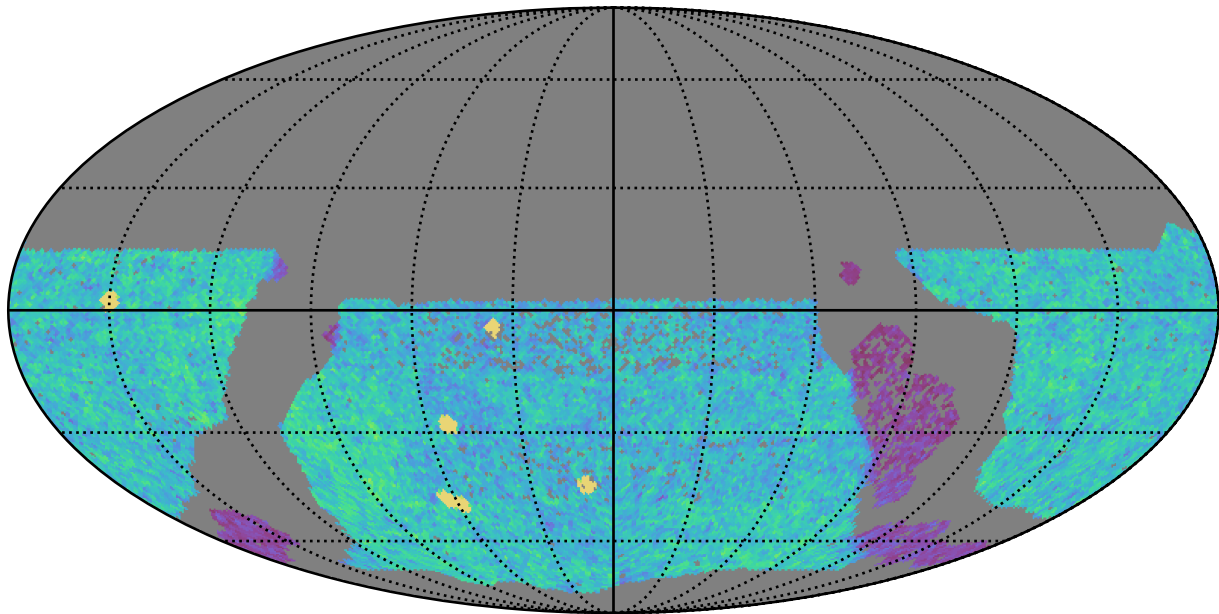
too_elab_r256_d2_griz_v3.4_10yrs WFD u band: NVisits
