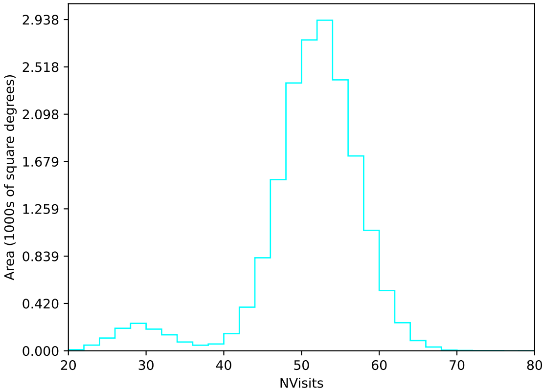
too_elab_r256_d2_griz_v3.4_10yrs WFD u band: NVisits
