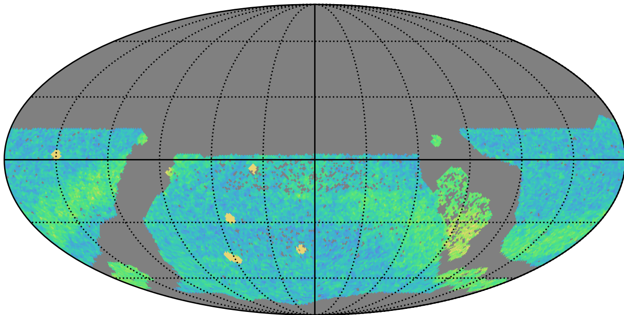
too_elab_r256_d2_griz_v3.4_10yrs WFD r band: NVisits
