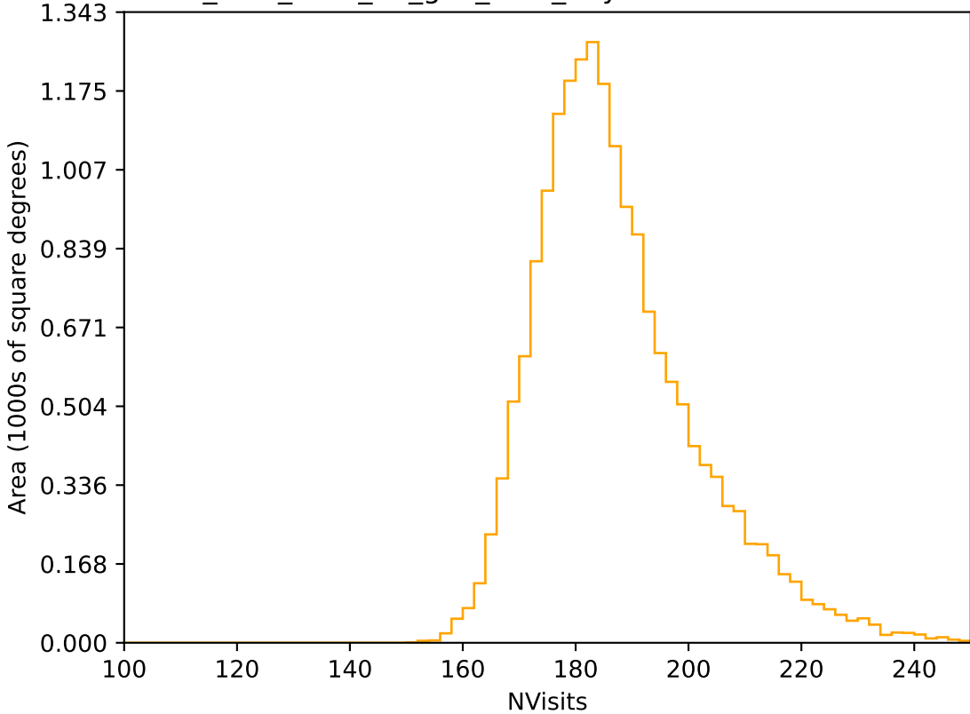
too_elab_r256_d2_griz_v3.4_10yrs WFD r band: NVisits
