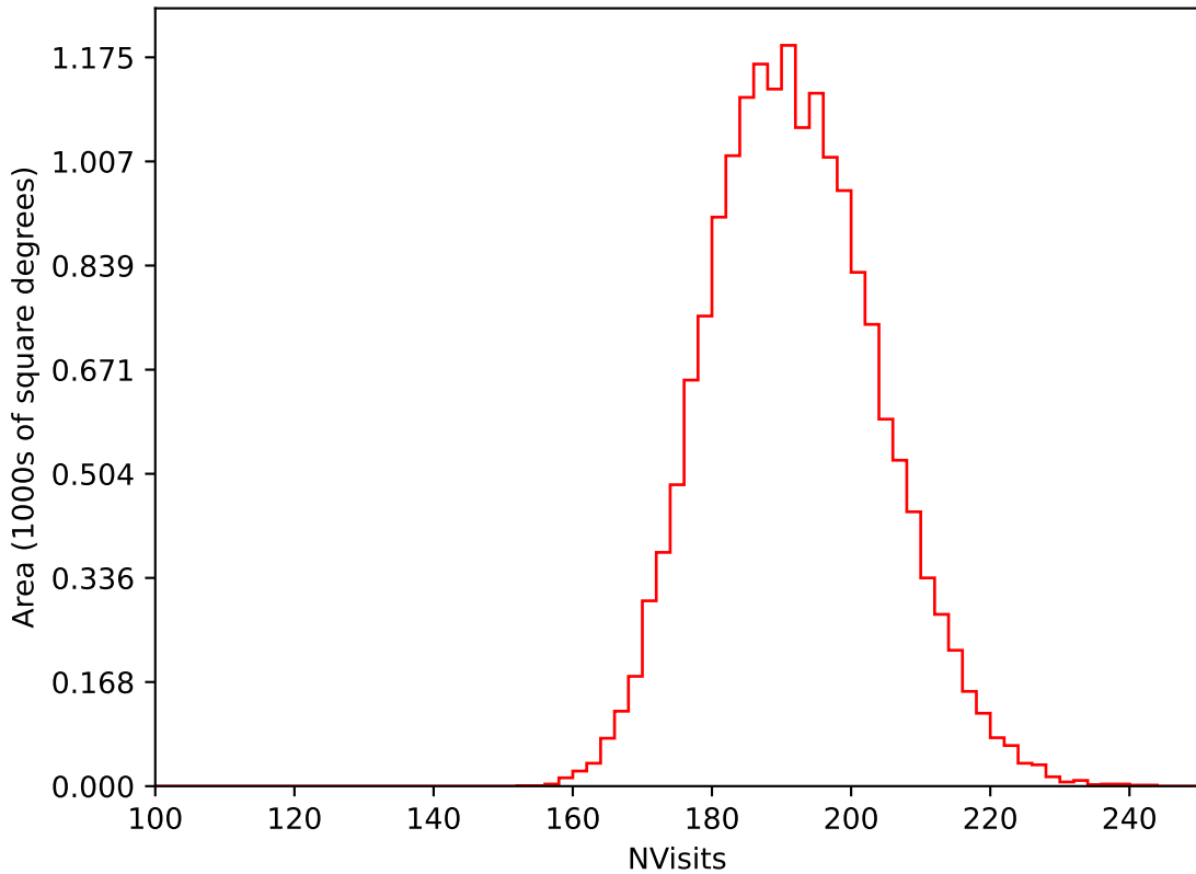
too_elab_r256_d2_griz_v3.4_10yrs WFD i band: NVisits
