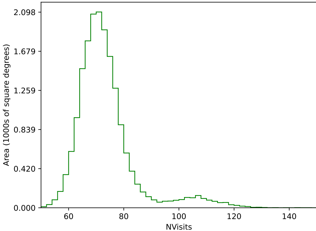
too_elab_r256_d2_griz_v3.4_10yrs WFD g band: NVisits
