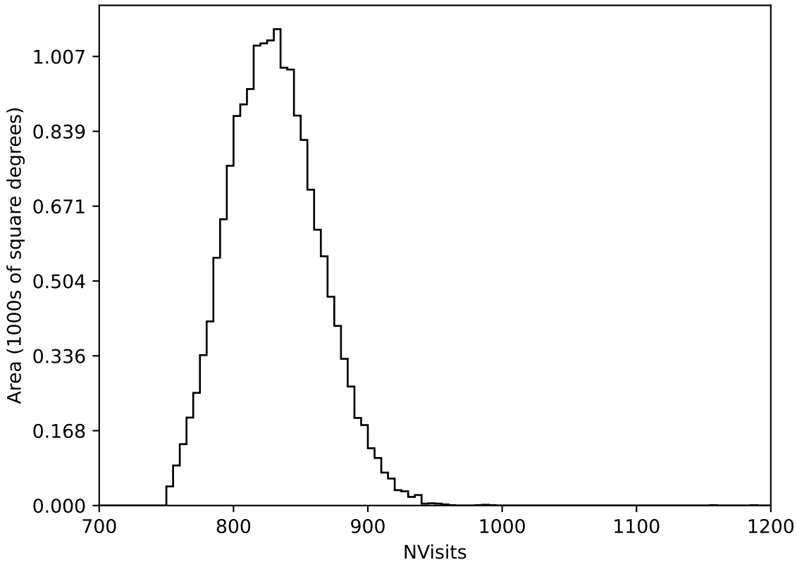
too_elab_r256_d2_griz_v3.4_10yrs WFD all bands: NVisits
