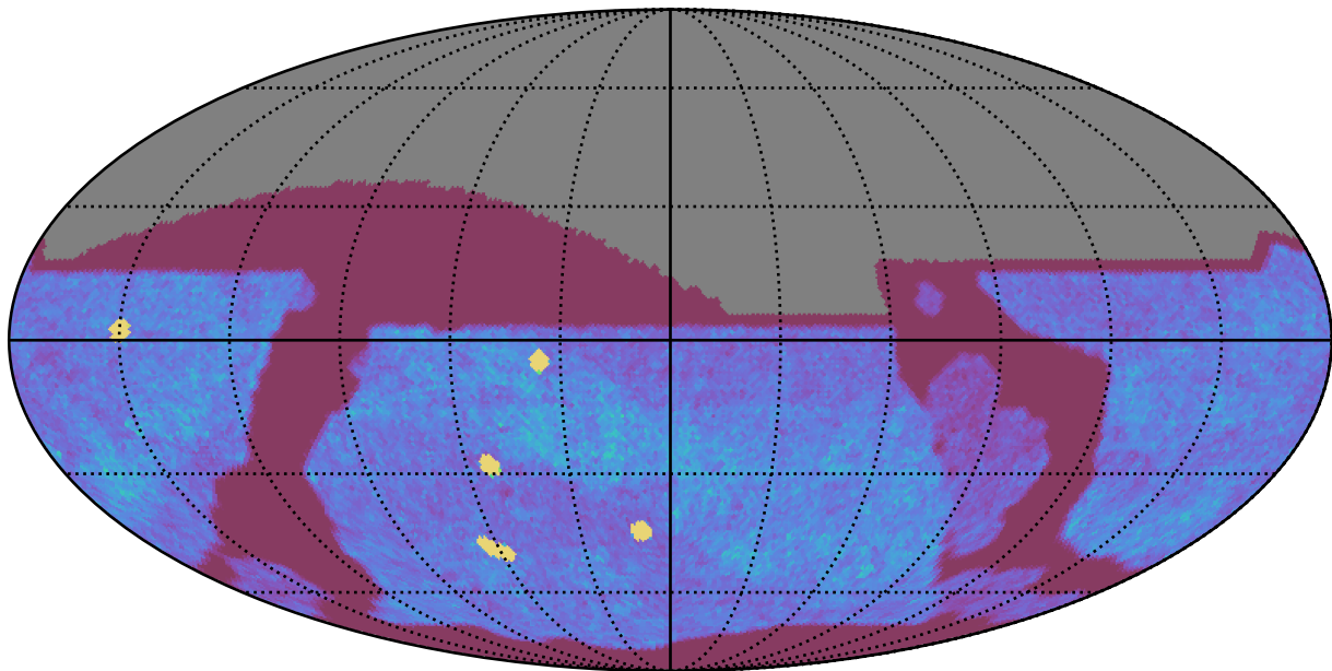
too_elab_r256_d2_griz_v3.4_10yrs All sky z band: NVisits
