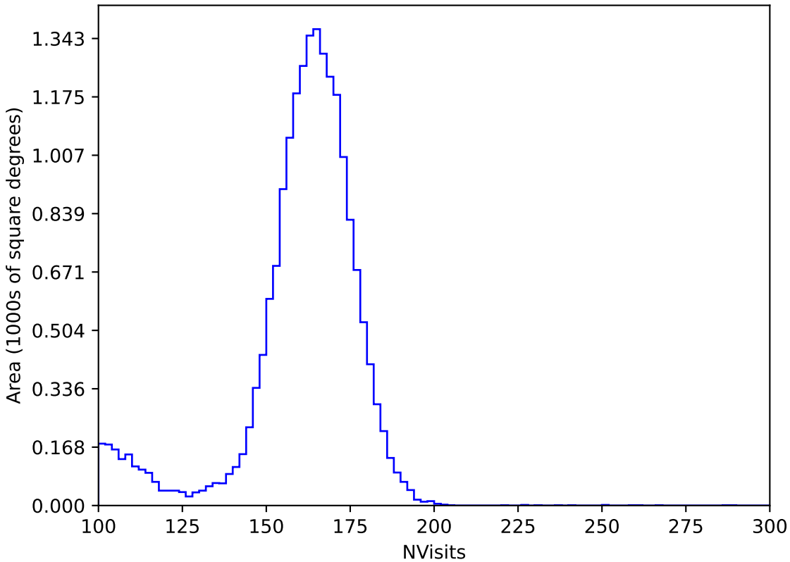
too_elab_r256_d2_griz_v3.4_10yrs All sky y band: NVisits
