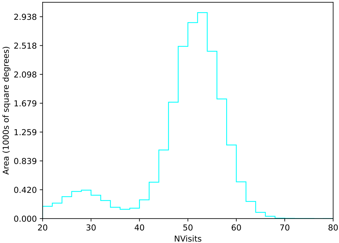
too_elab_r256_d2_griz_v3.4_10yrs All sky u band: NVisits
