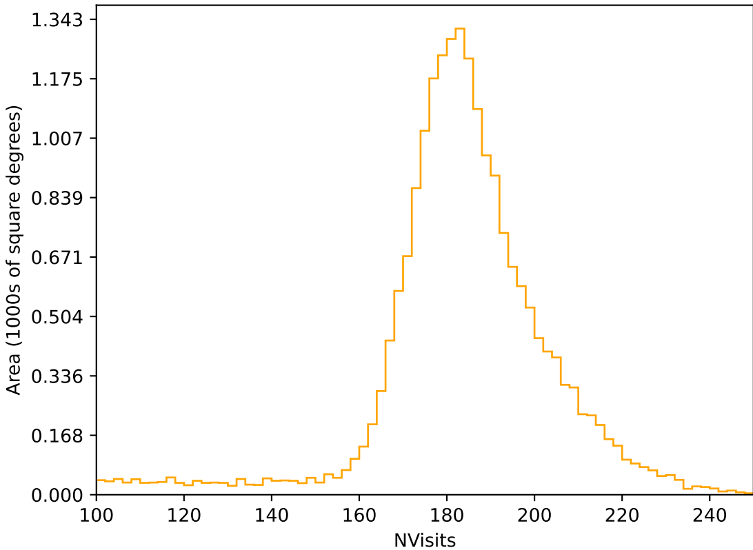
too_elab_r256_d2_griz_v3.4_10yrs All sky r band: NVisits
