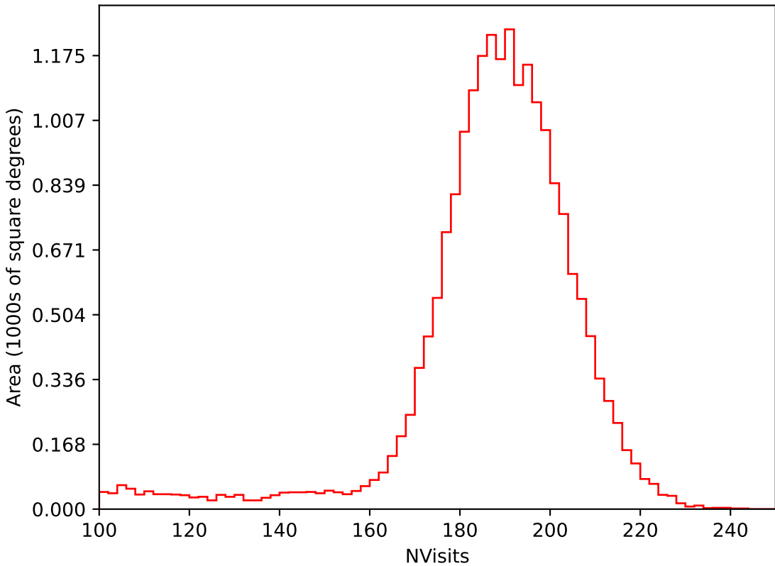
too_elab_r256_d2_griz_v3.4_10yrs All sky i band: NVisits
