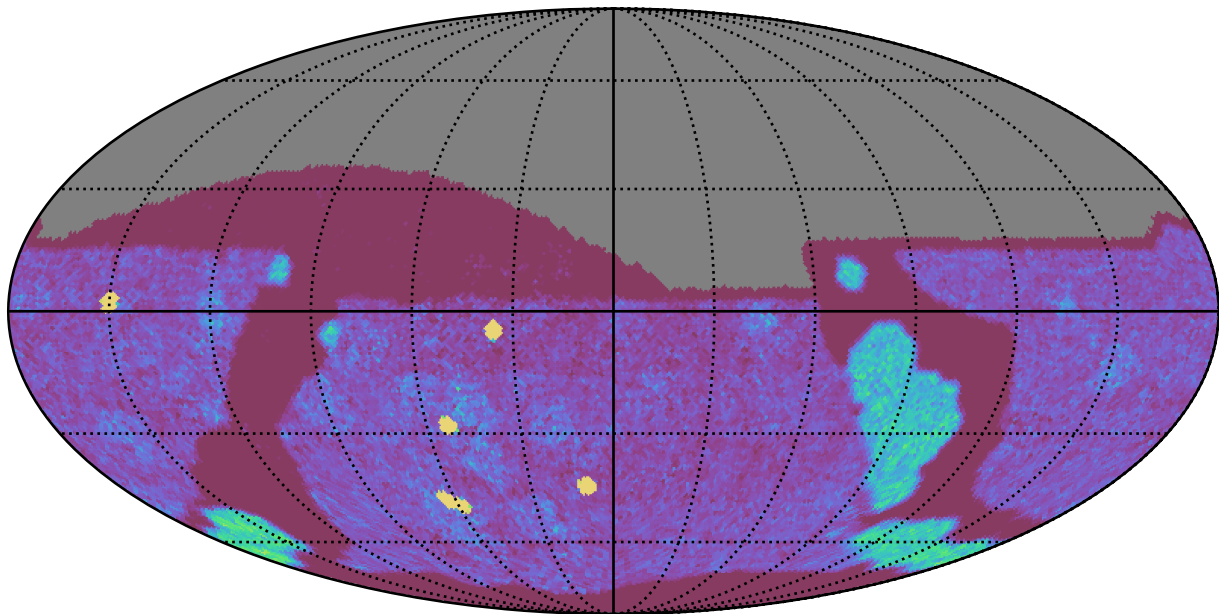
too_elab_r256_d2_griz_v3.4_10yrs All sky g band: NVisits
