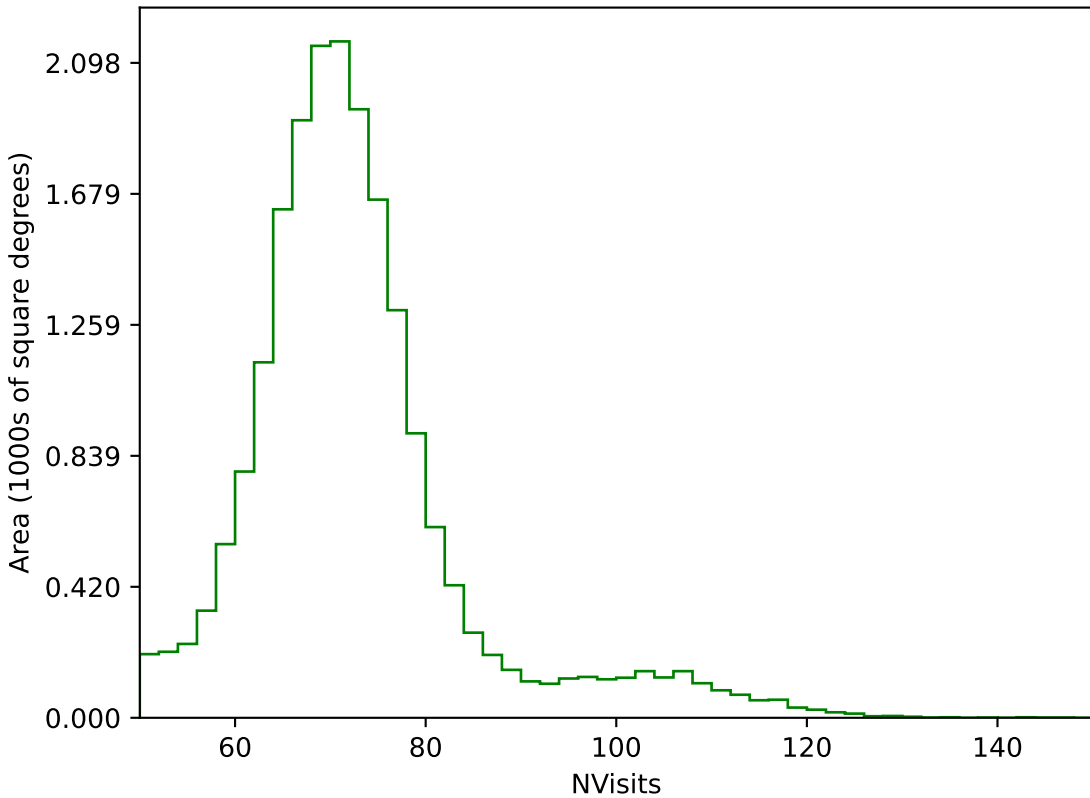
too_elab_r256_d2_griz_v3.4_10yrs All sky g band: NVisits
