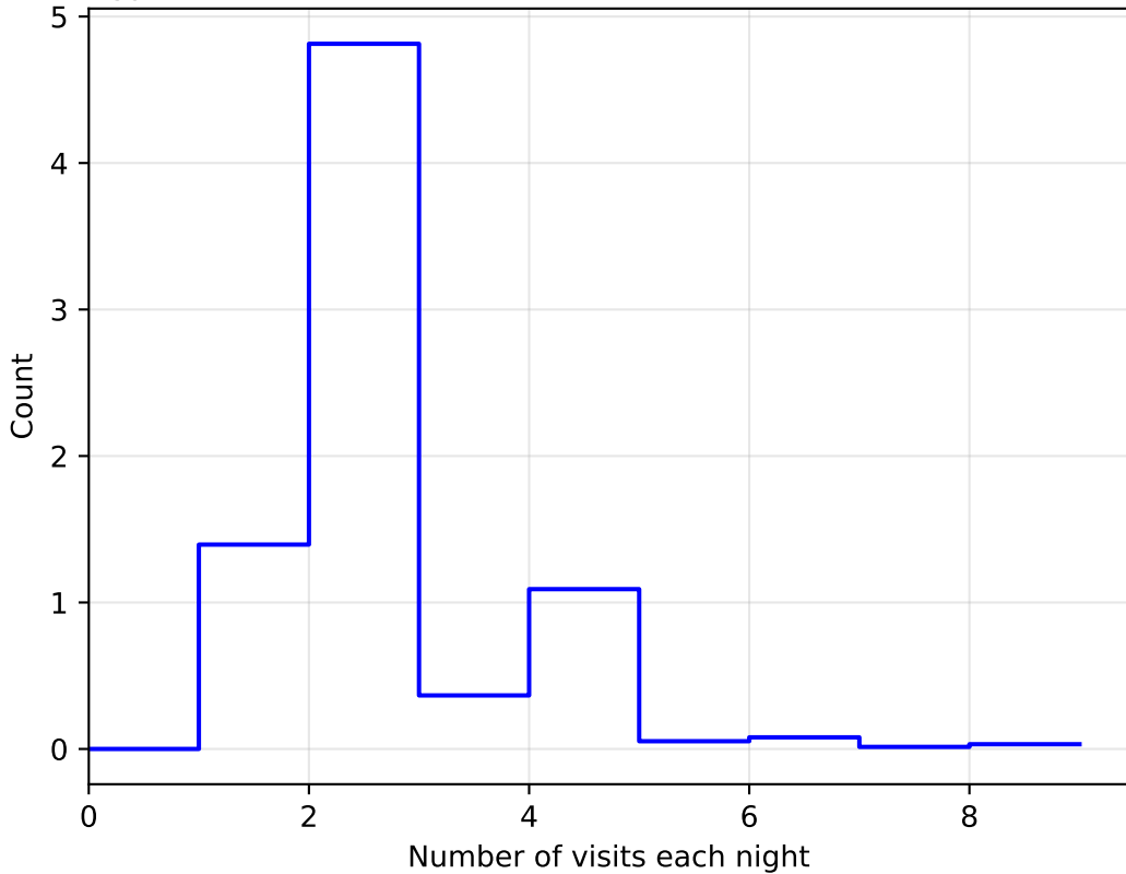
too_elab_r256_d2_griz_v3.4_10yrs WFD: NVisitsPerNight
