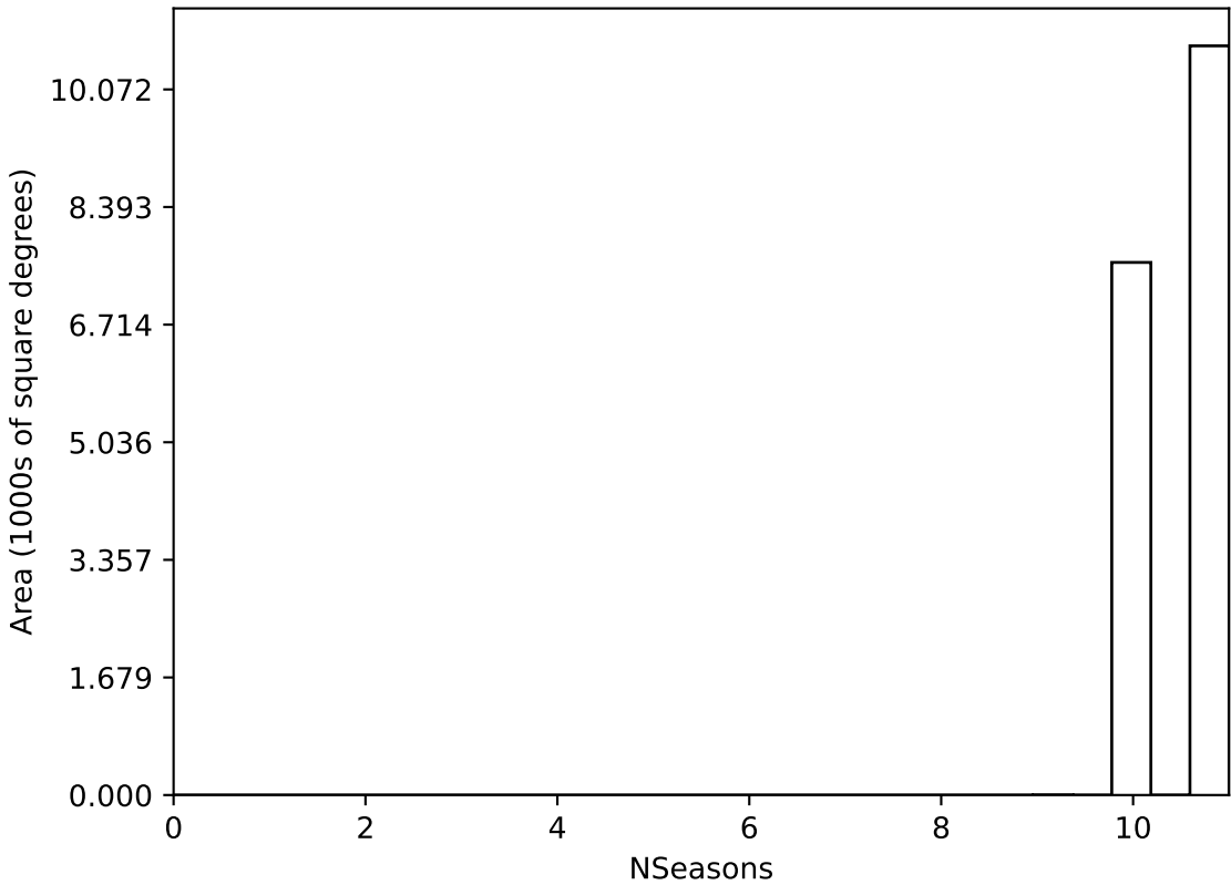
too_elab_r256_d2_griz_v3.4_10yrs WFD all bands: NSeasons
