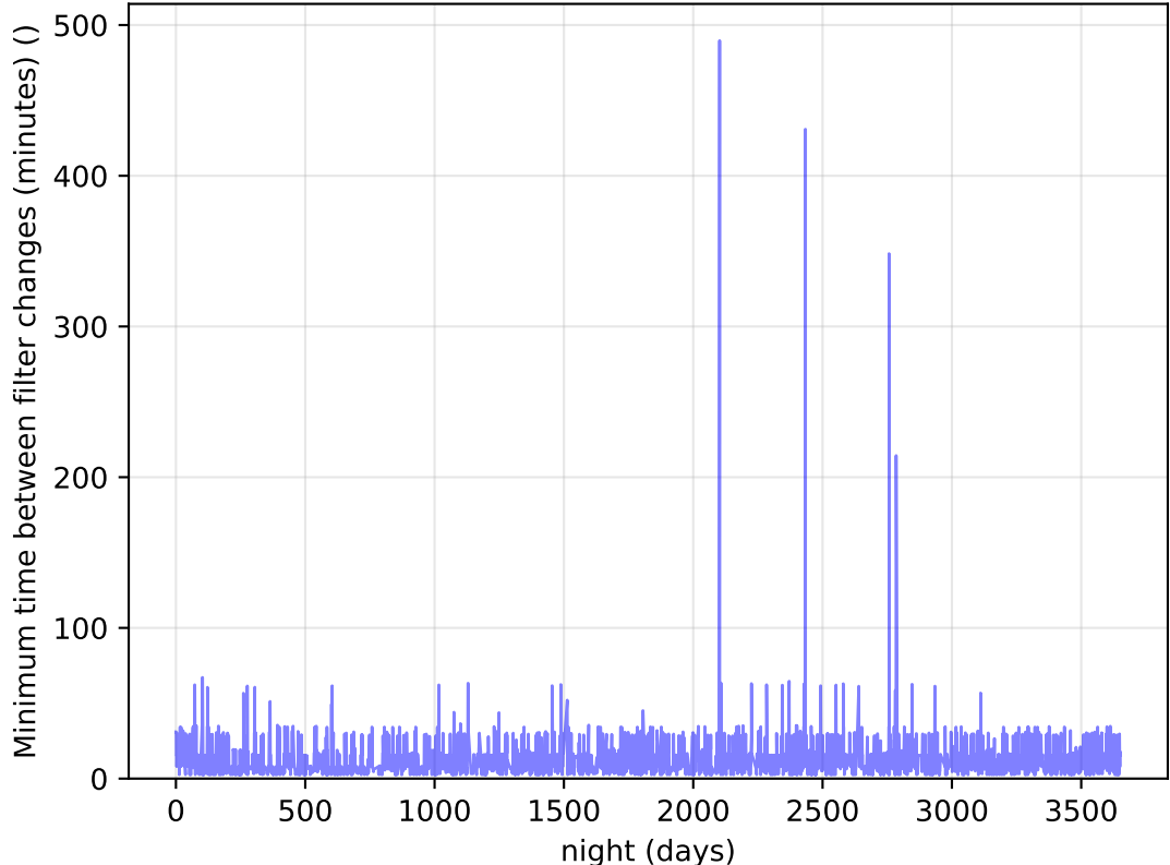
too_elab_r256_d2_griz_v3.4_10yrs Per Night: Minimum time between filter changes (minutes)
