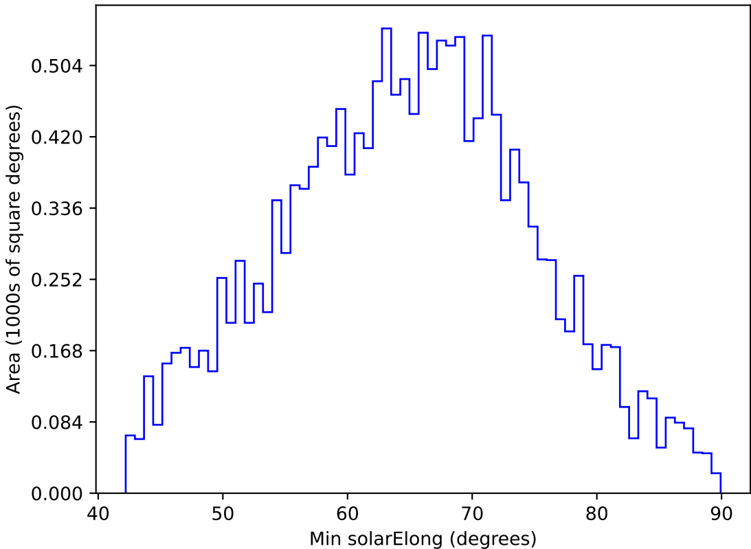
too_elab_r256_d2_griz_v3.4_10yrs WFD y band: Min solarElong
