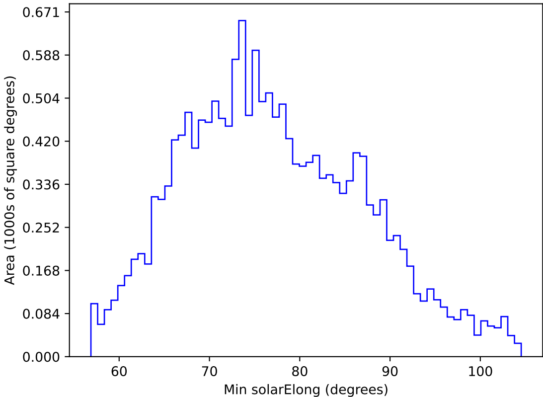
too_elab_r256_d2_griz_v3.4_10yrs WFD u band: Min solarElong
