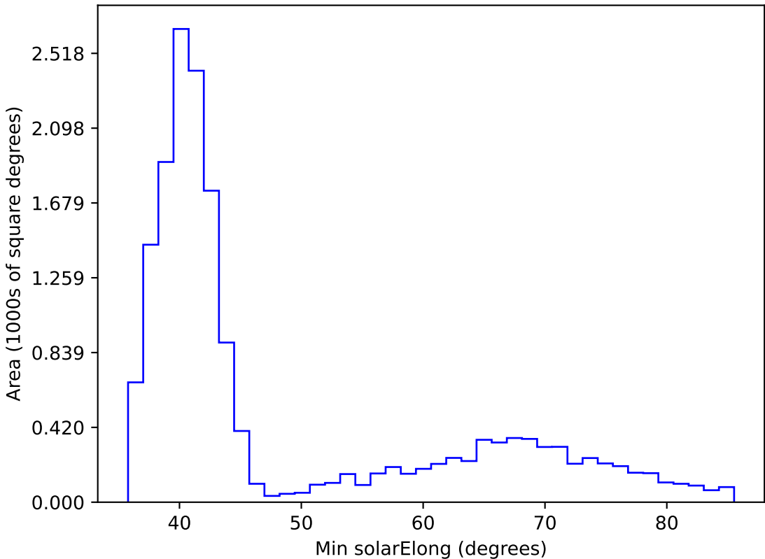
too_elab_r256_d2_griz_v3.4_10yrs WFD i band: Min solarElong
