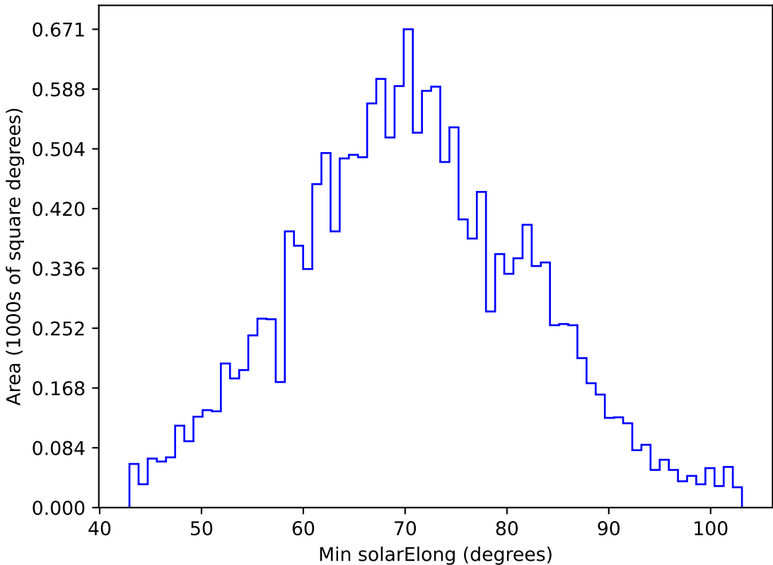
too_elab_r256_d2_griz_v3.4_10yrs WFD g band: Min solarElong
